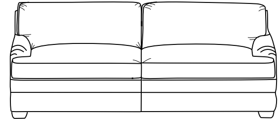
10-127 - Sofa Knife edge back pillows with legs 10-127-60 60 x 39 x 37 SW: 48 SD: 22 SH: 20 AH: 24 10-127-72 72 x 39 x 37 SW: 60 SD: 22 SH: 20 AH: 24
