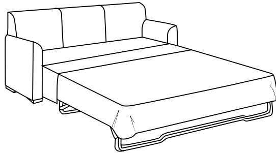
10-329 - Sleeper Tight back with built to floor or small leg 10-329-72 - Double 72 x 39 x 34 AH: 26 SH: 20 SD: 22 10-329-84 - Queen 84 x 39 x 34 AH: 26 SH: 20 SD: 22
